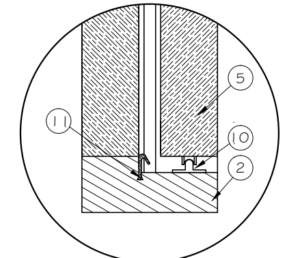
DETAIL B
